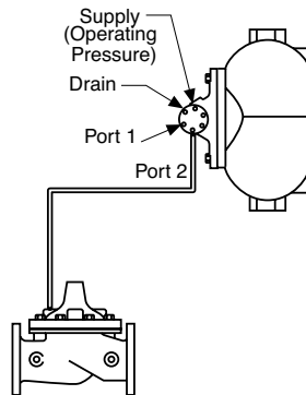
Float Down Closes Valve
