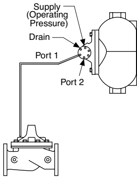
Float Up Closes Valve
