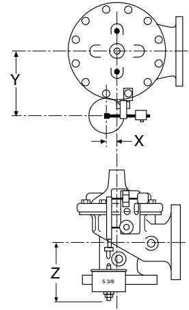
ANGLE 124-02 8" to 16"
