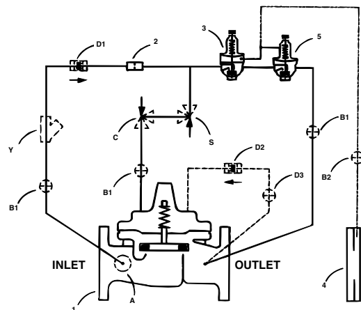
The "D" feature on a vertically installed 6" and larger valves must be horizontally installed.
