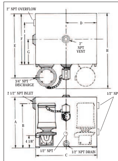
G SERIES 30-120 GALLON TANKS
