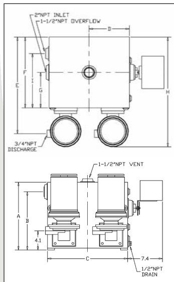
G SERIES (DUPLEX) 15 GALLON TANK
