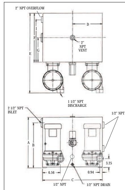
J SERIES 30-120 GALLON TANKS
