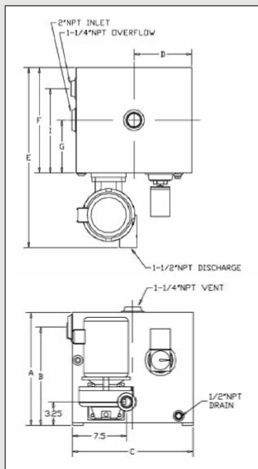
J SERIES (SIMPLEX) 15 GALLON TANK
