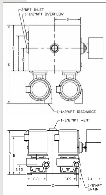
J SERIES (DUPLEX) 15 GALLON TANK
