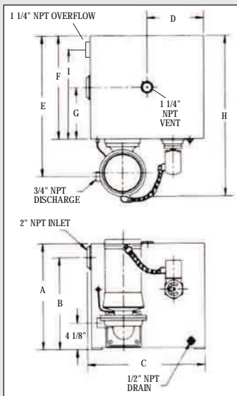
G SERIES (SIMPLEX) 8 OR 15 GALLON TANK
