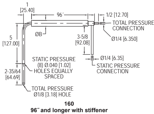
Standard Model 160 pitot tube
