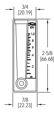
Model MMF-10 with 1-1/2" scale, no valve.
